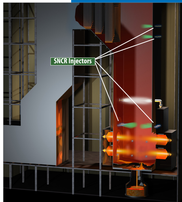
SNCR Injection Process
